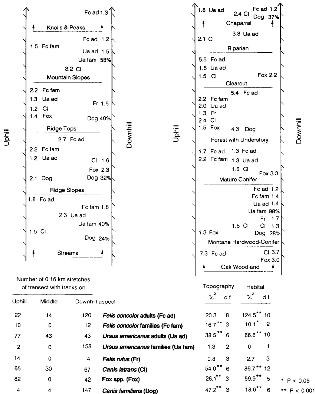
Fig. 3. Preferences, M_{y|x} , for uphill, middle or downhill aspects of the road used by carnivore species as topography and habitats changed. Black bear families and dog used the downhill side of the road overwhelmingly so their preferences were expressed by percentages.
